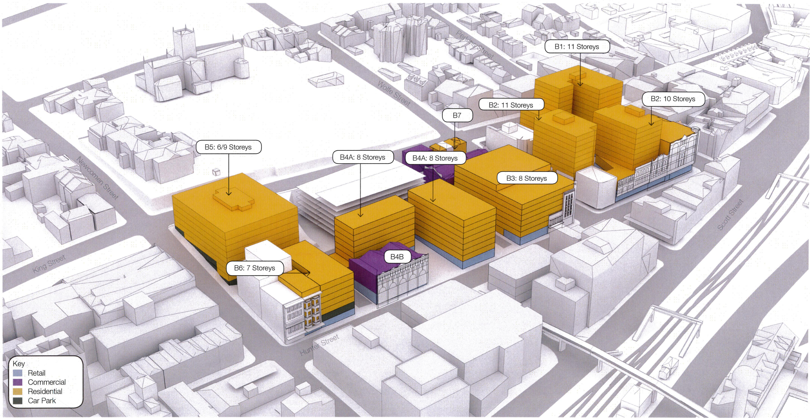
Figure 5.17.1 Massing Diagram 2
